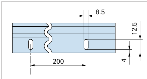
Standard holes for CM14 / CM15
